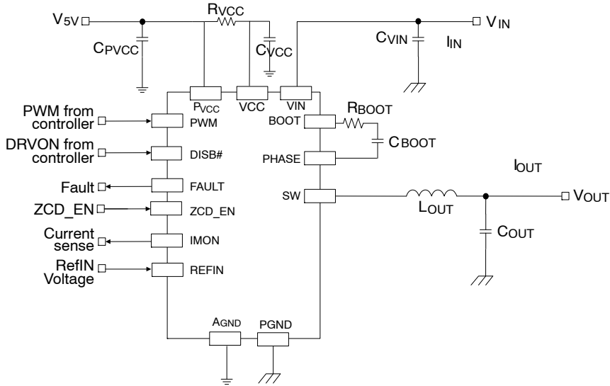
Figure 1. Application Diagram
