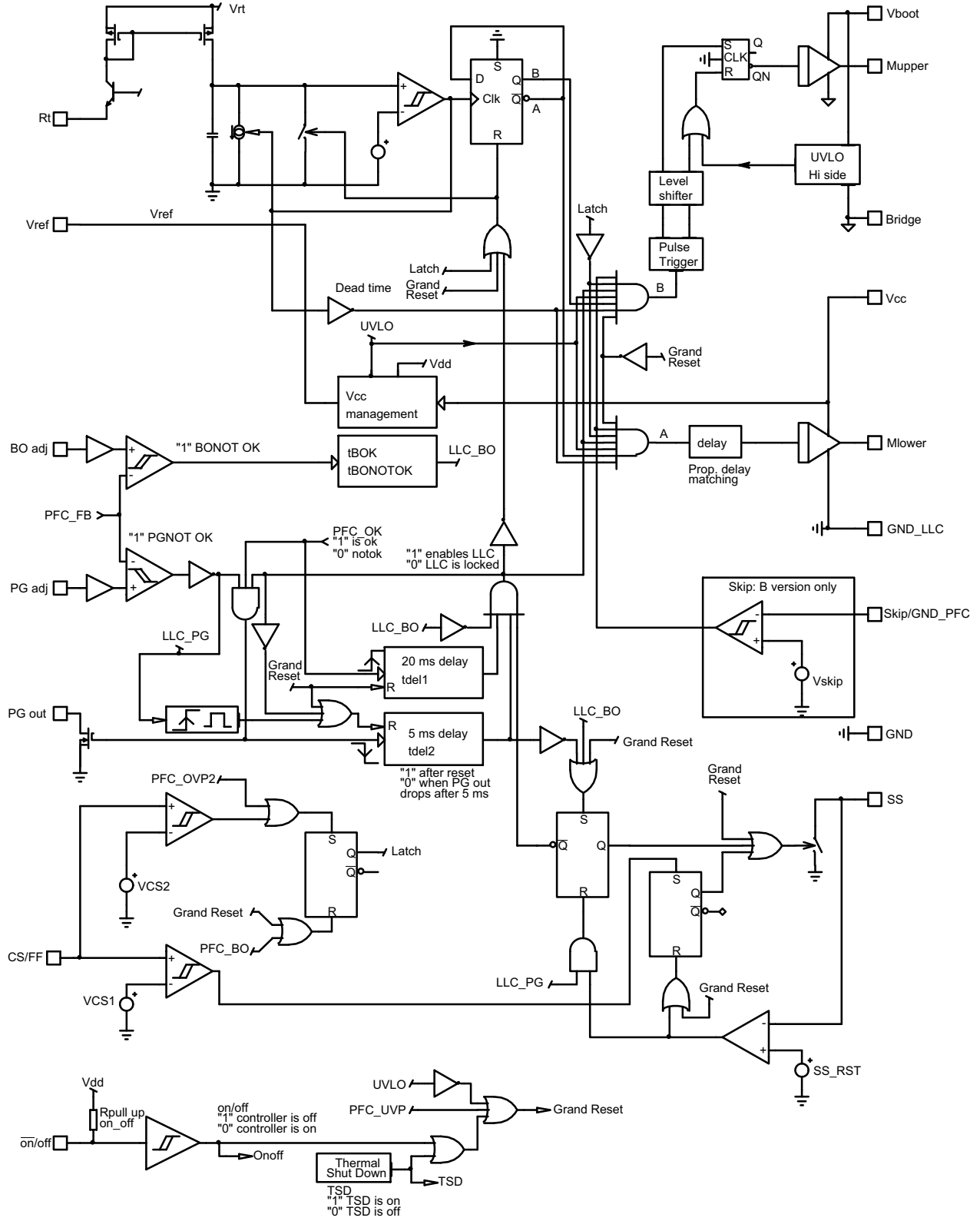
Figure 5. Internal LLC Block Diagram
