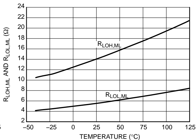
Figure 35. R_{LOH,ML} and R_{LOL,ML} vs. Temperature
