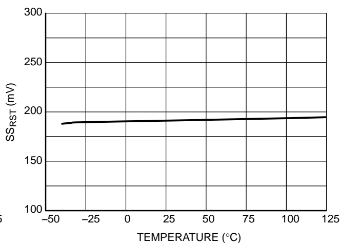
Figure 33. SS_{RST} vs. Temperature
