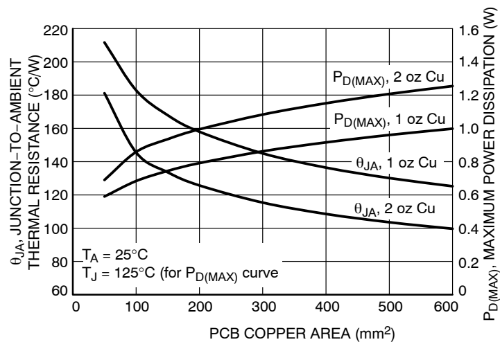
Figure 30. \theta_{JA} and P_{D(MAX)} vs. Copper Area
