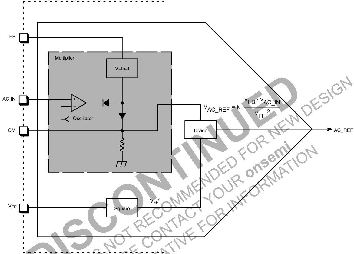
Figure 67. Reference Generator
