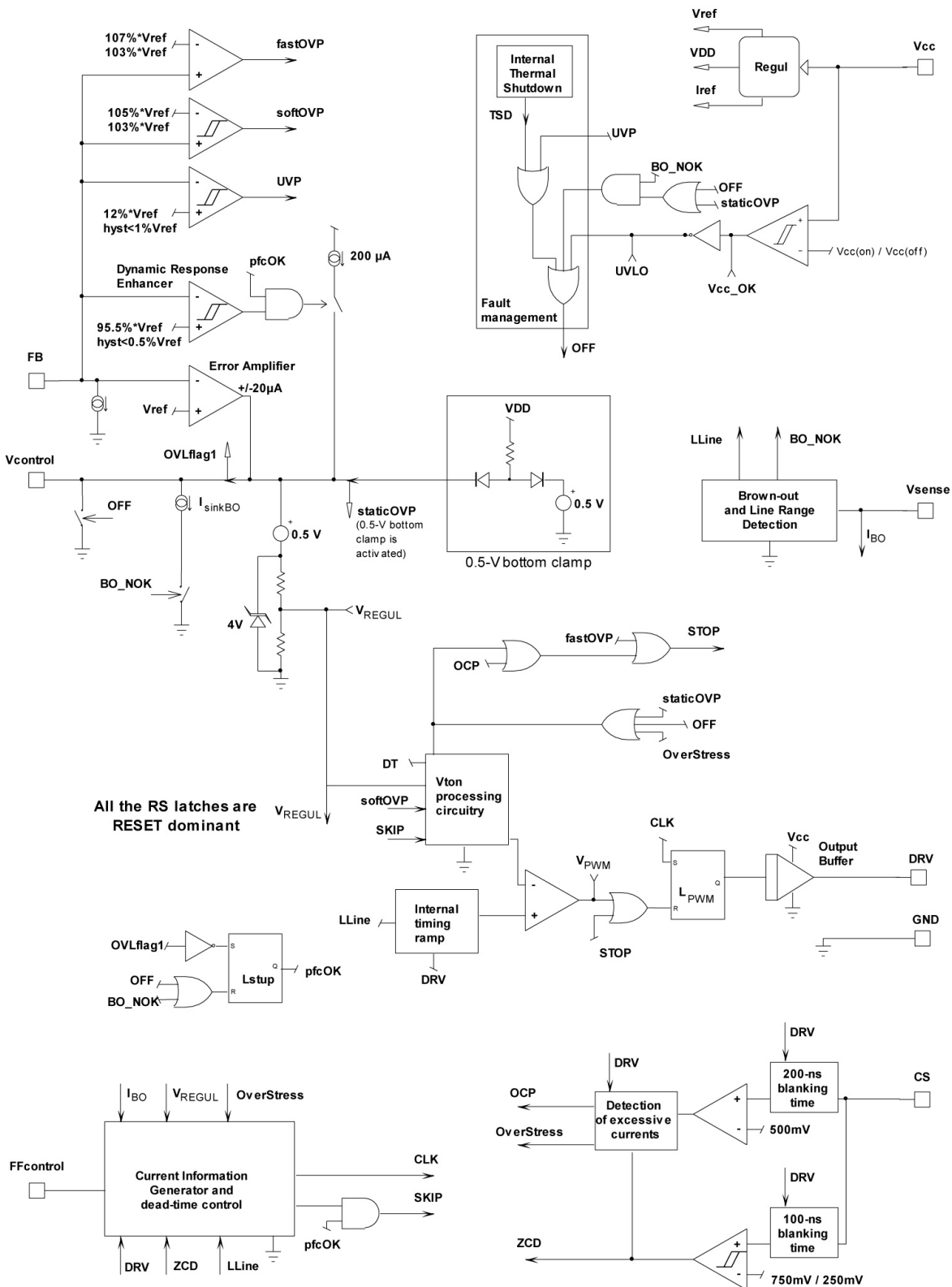
Figure 2. Block Diagram
