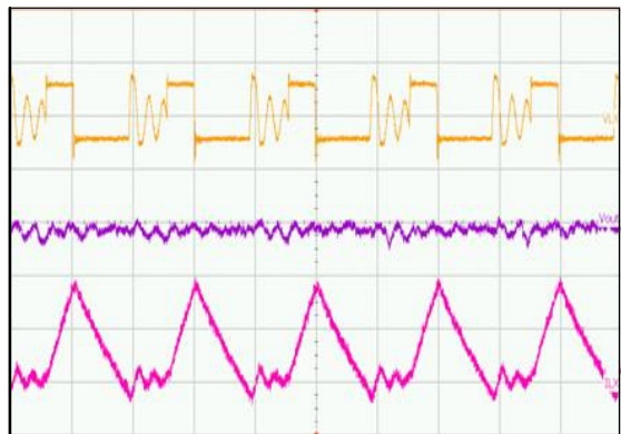
(VIN = 5 V, VOUT = 1.8 V, IOU = 150 A) Upper Trace: LX Pin Switching Waveforms, 5 V / div Middle Trace: Output Voltage, 20 mV / div Lower Trace: Inductor Current, 200 mA / div Time = 500 ns / div
