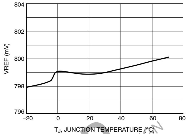
Figure 4. Reference Voltage
