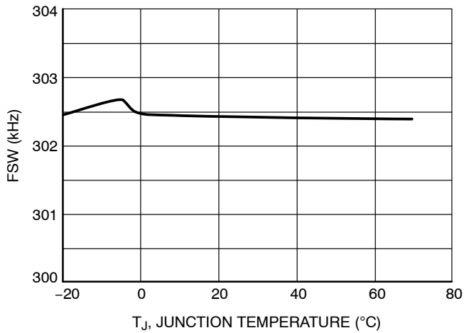
Figure 3. Oscillator Frequency
