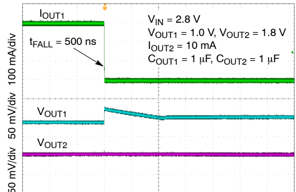
Figure 41. Load Transient Response – 1.0 V – Falling Edge, I_{OUT1} = 300\text{ mA} to 100\text{ μA}
