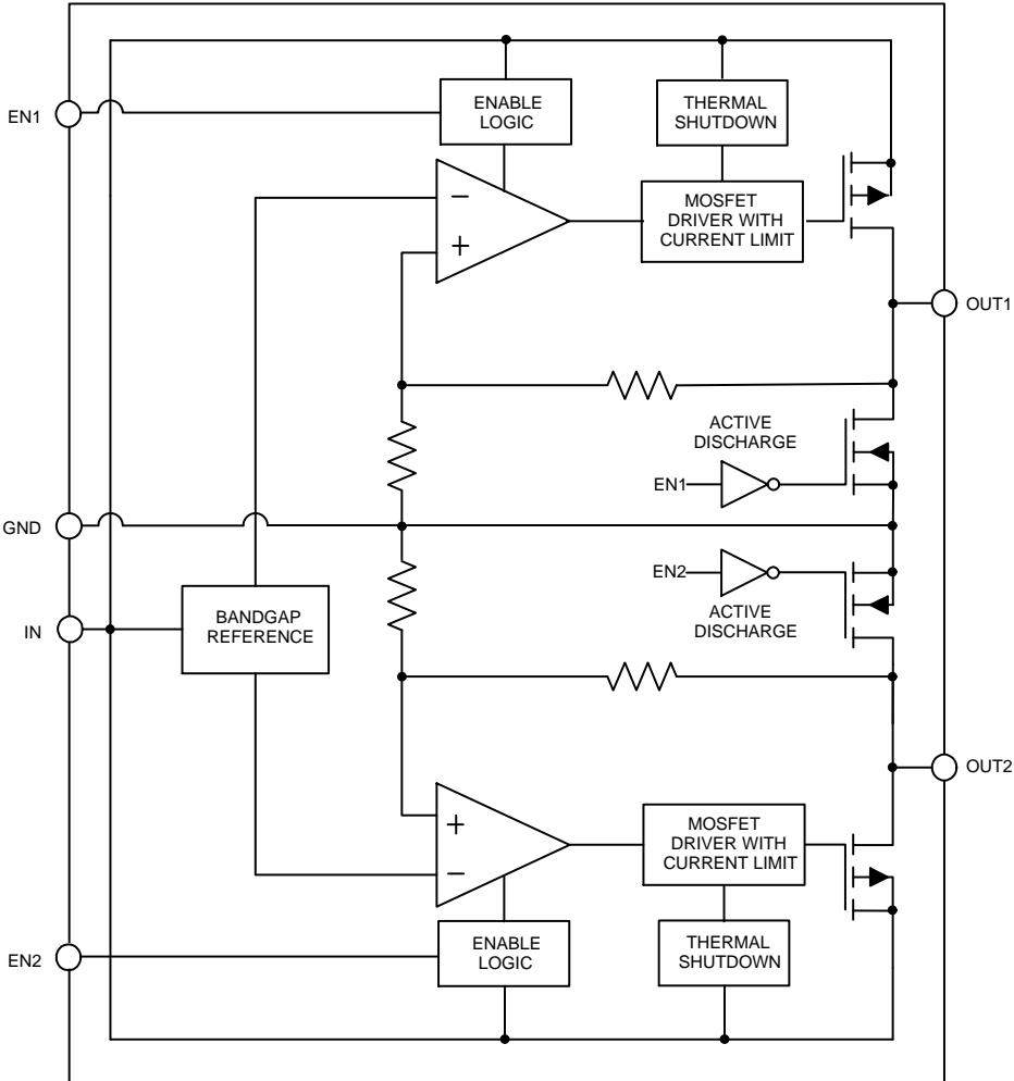
Figure 2. Simplified Schematic Block Diagram
