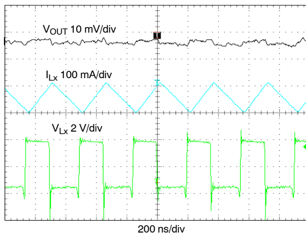
Figure 27. PWM Switching Waveform ( V_{IN} = 3.6 V, V_{OUT} = 1.2 V, I_{OUT} = 600 mA)
