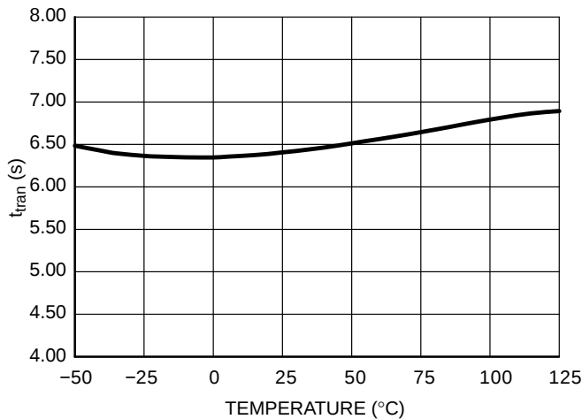
Figure 43. Transient Peak Power Timer Timer Duration t_{tran}
