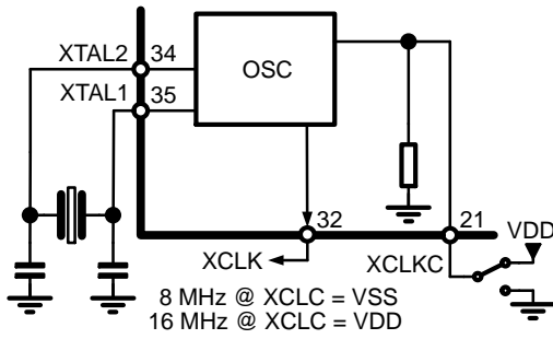
Figure 11. XTAL Oscillator
