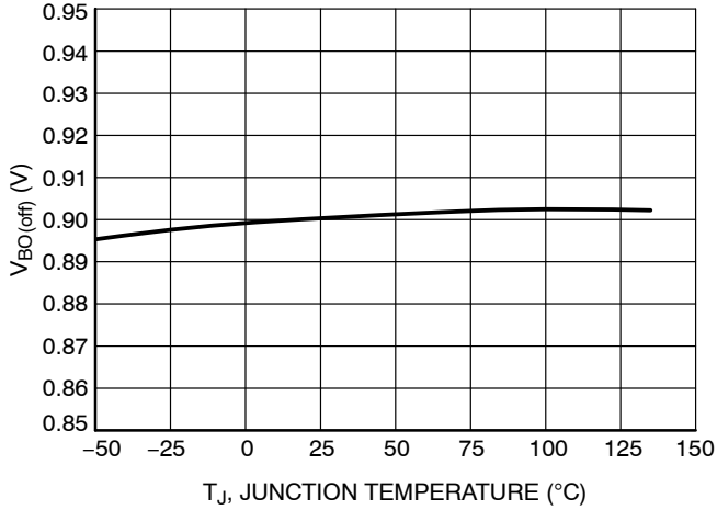
Figure 56. Brown-out OFF Level vs. Temperature
