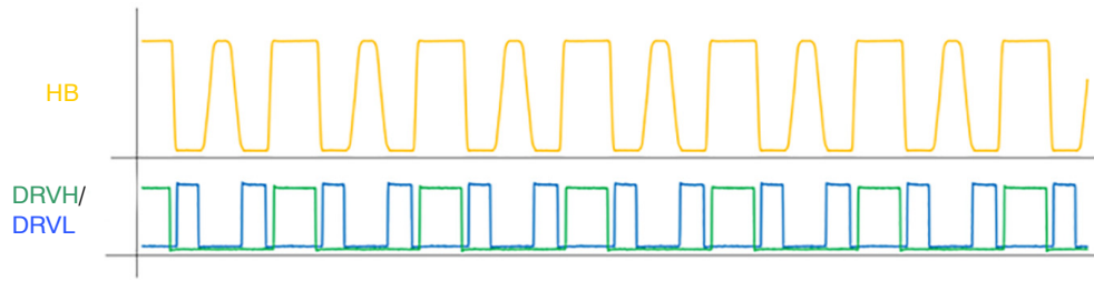
Figure 79. Light-load Operation
