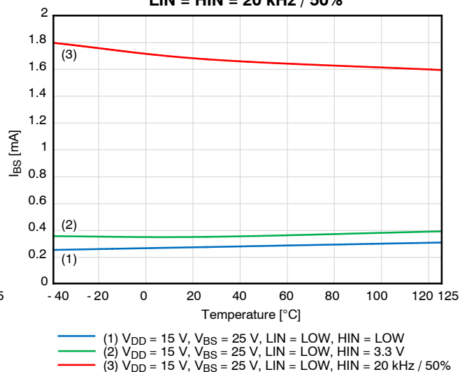
Figure 13. I_{BS} Supply Current V_{BS} = 25 V
