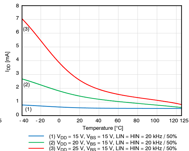
Figure 11. I_{DD} Supply Current V_{DD} = 15 – 25 V, LIN = HIN = 20 kHz / 50%
