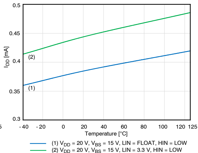
Figure 9. I_{DD} Supply Current V_{DD} = 20 V
