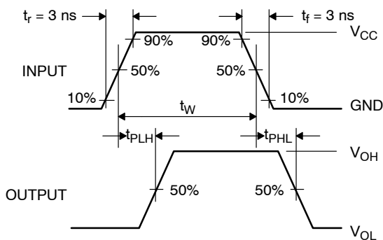
Figure 6. AC Waveforms
