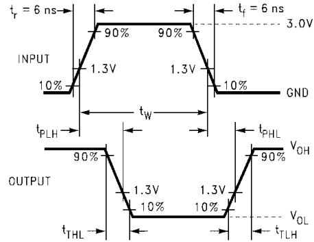
Figure 6. AC Waveforms
