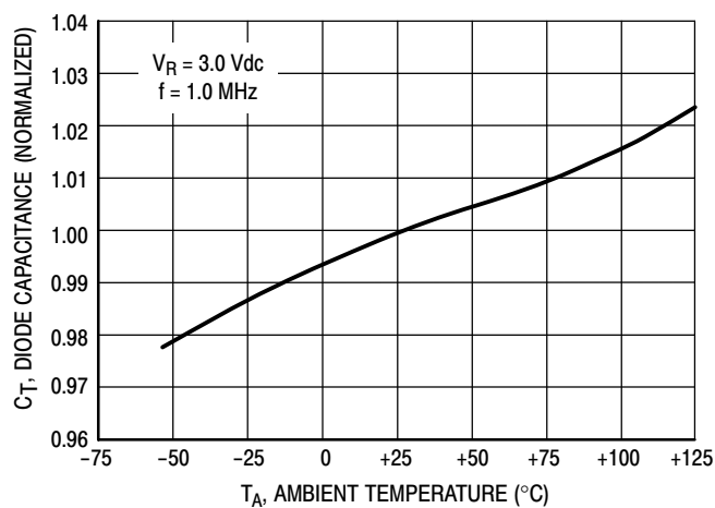
Figure 4. Diode Capacitance
