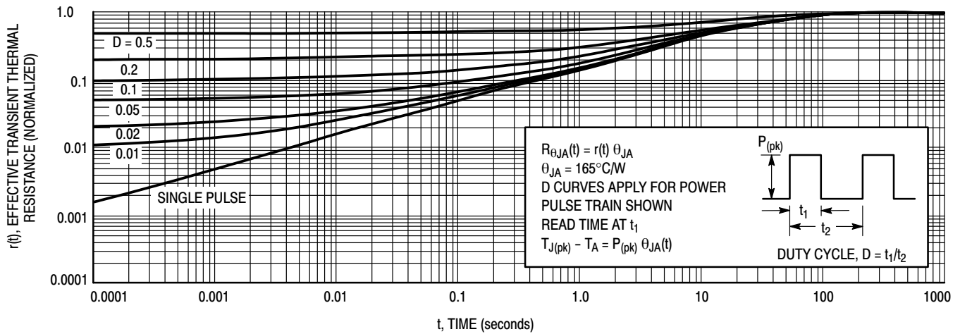
Figure 12. Thermal Response
