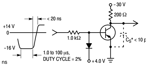
Figure 2. Turn–Off Time
