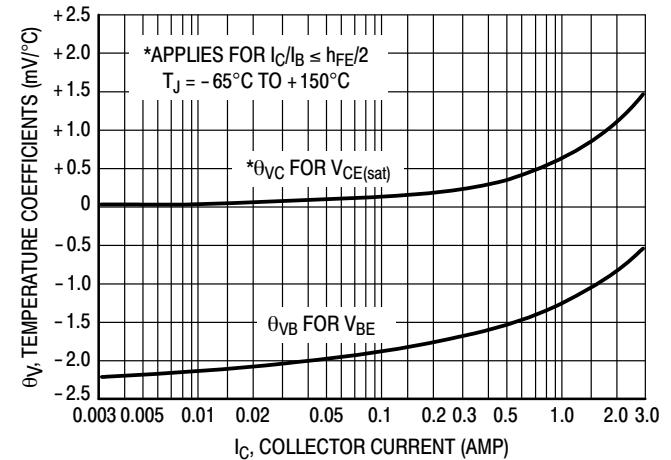
Figure 11. Temperature Coefficients
