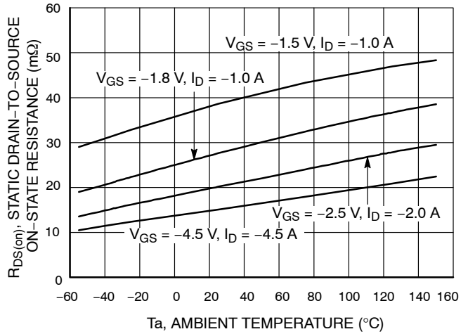
Figure 5. R_{DS(on)} - T_a
