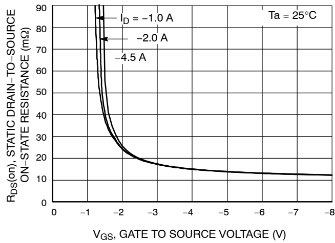
Figure 4. R_{DS(on)} - V_{GS}
