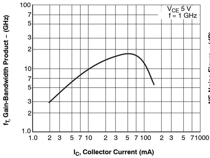
Figure 7. f_T - I_C
