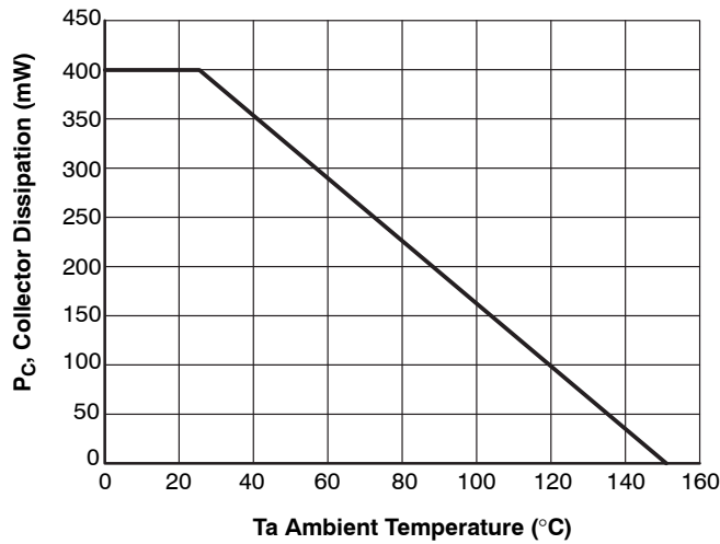
Figure 9. P_C - T_a
