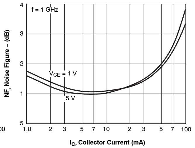
Figure 8. NF - I_C
