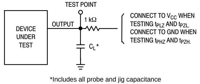
Figure 6. Test Circuit
