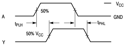
Figure 3. Switching Waveforms
