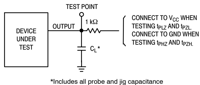
Figure 7. Test Circuit
