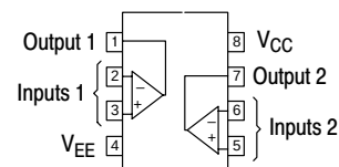
(Dual, Top View)
