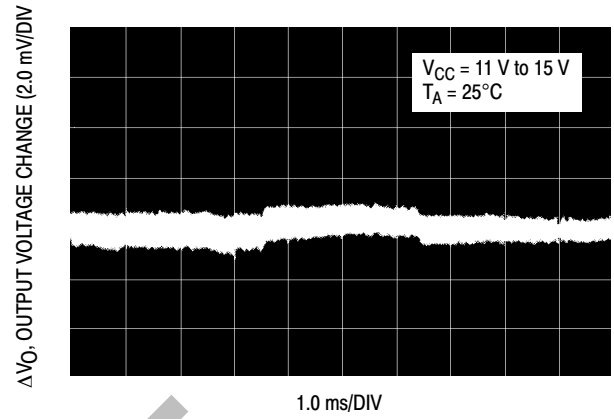
Figure 11. Reference Line Regulation
