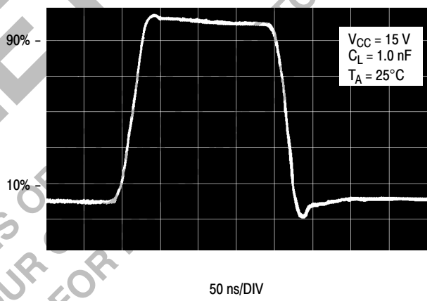
Figure 13. Output Waveform
