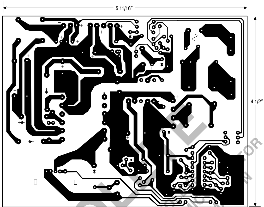
Circuit View
