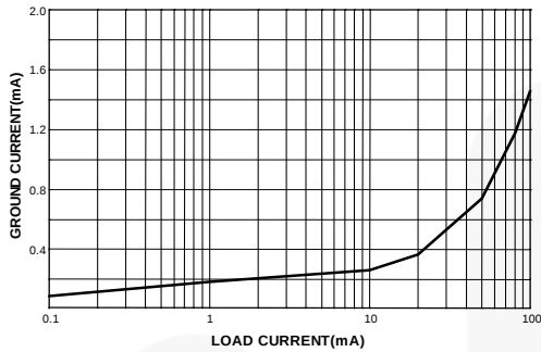
Figure 2. Quiescent Current
