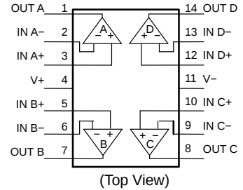
TSSOP-14
