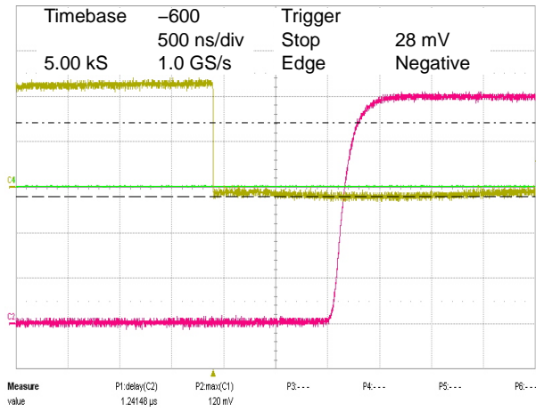
Figure 13. 10 mV Overdrive
