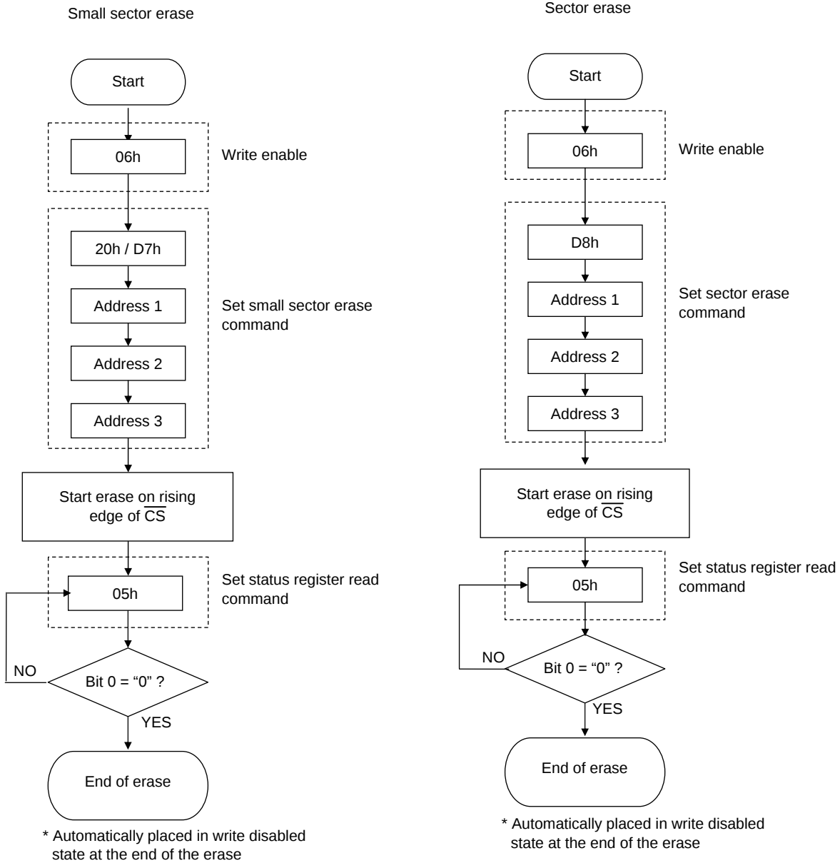
Figure 20 Erase Flowcharts
