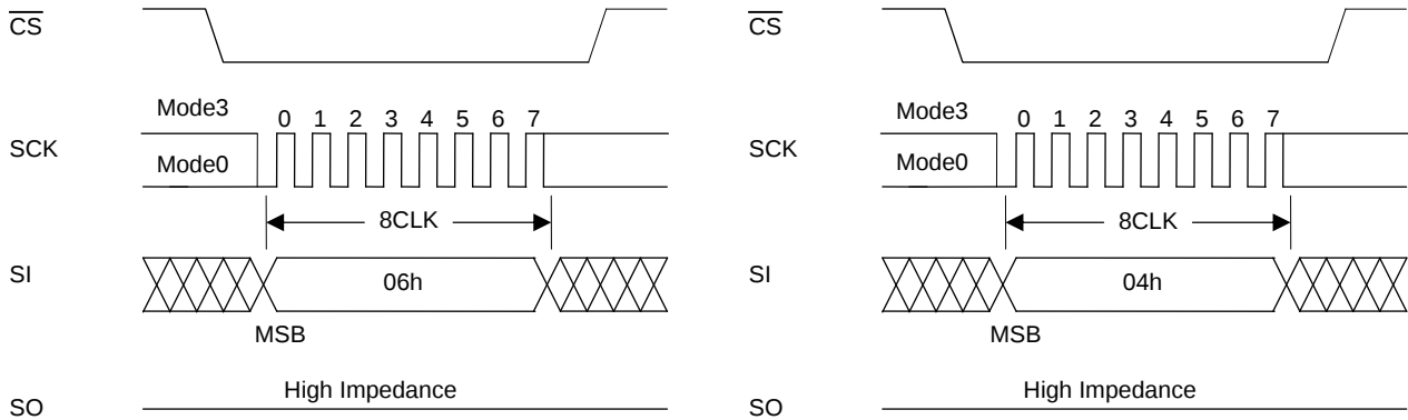
Figure 7 Write Enable
