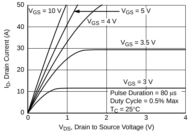
Figure 8. Saturation Characteristics
