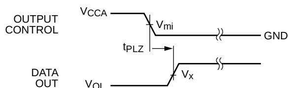
Figure 10. 3-STATE Output High Enable Time (17)
