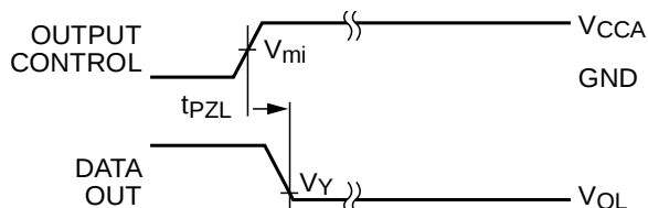
Figure 9. 3-STATE Output Low Enable Time (17)
