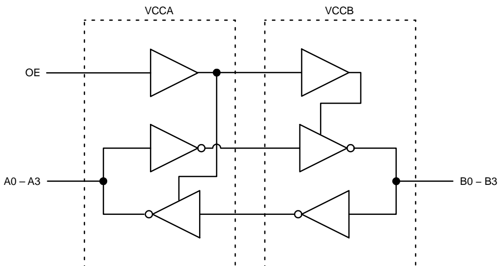
Figure 1. Functional Diagram
