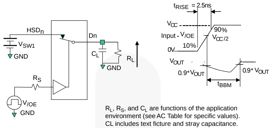
Figure 13. Break-Before-Make Interval Timing
