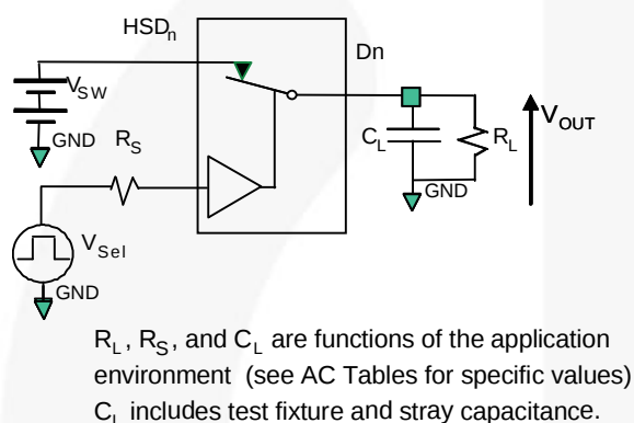
Figure 7. AC Test Circuit Load
