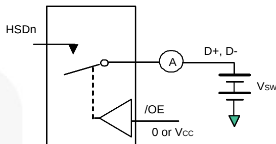
Figure 6. Off/On Leakage
