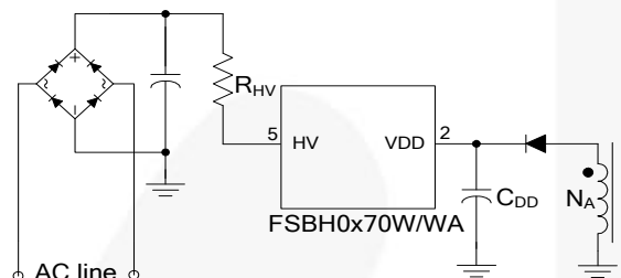
Figure 22. Startup Circuit
