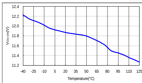
Figure 8. V_{DD-ON} vs. Temperature
