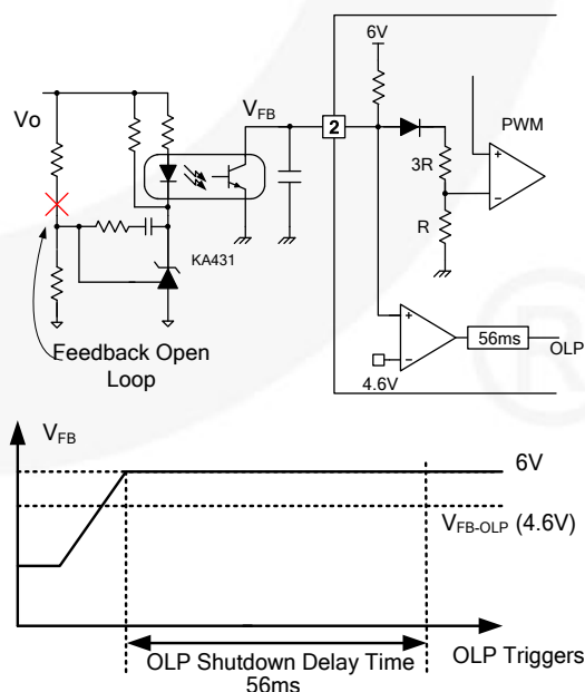
Figure 29. OLP Operation
