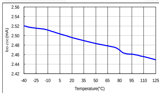
Figure 18. I_{D-ZDC} vs. Temperature
