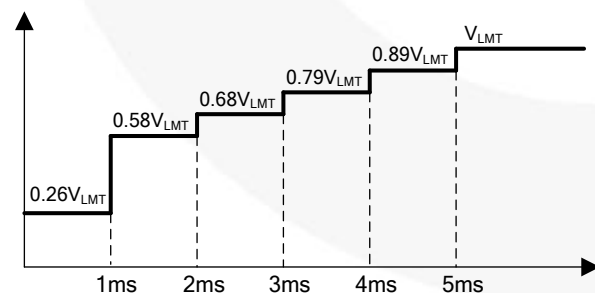
Figure 23. Soft-Start Function
