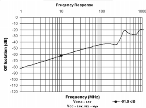
Figure 7. Off Isolation
