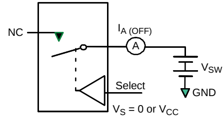
Figure 3. Off Leakage
