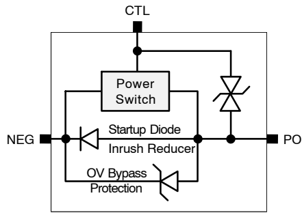
Figure 1. Block Diagram
