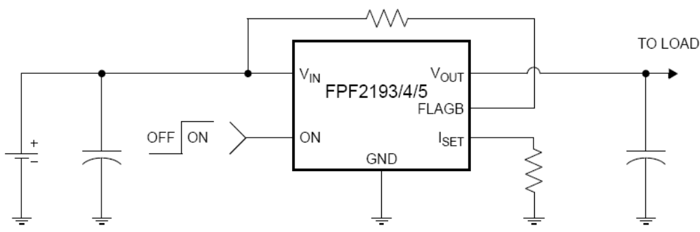
Figure 1. Typical Application
