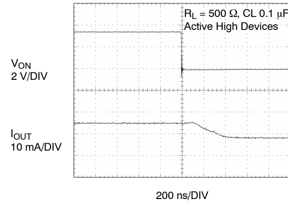
Figure 19. T_{OFF} Response
