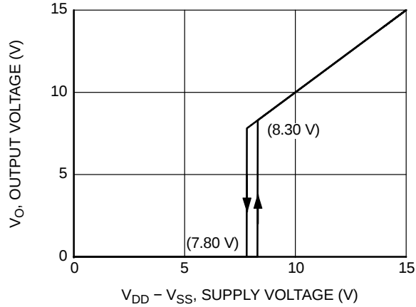
Figure 16. Under Voltage Lockout
