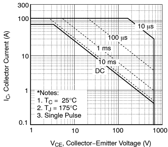
Figure 16. SOA Characteristics
