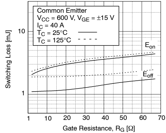
Figure 10. Switching Loss vs. Gate Resistance
