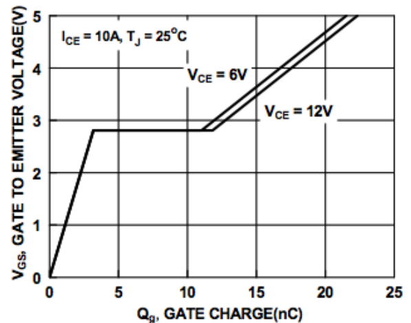
Figure 10. Gate Charge
