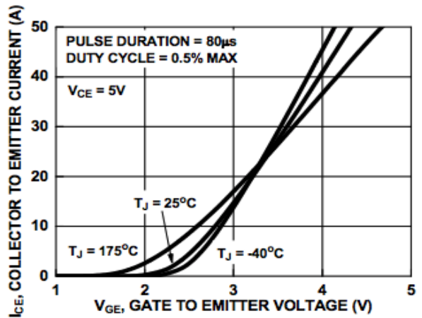
Figure 8. Transfer Characteristics
