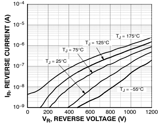
Figure 2. Reverse Characteristics
