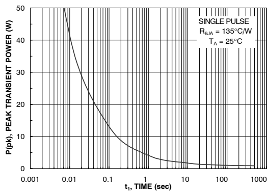
Figure 21. Single Pulse Maximum Power Dissipation
