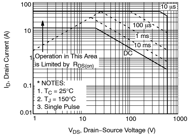
Figure 10. Maximum Safe Operating Area - FDP12N60NZ
