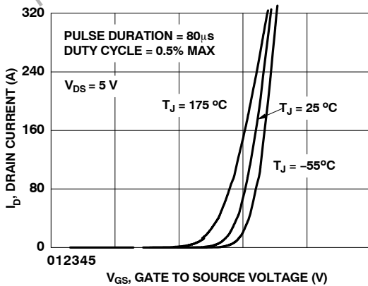
Figure 4. Transfer Characteristics
