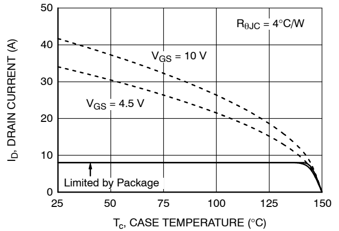
Figure 22. Maximum Continuous Drain Current vs. Case Temperature
